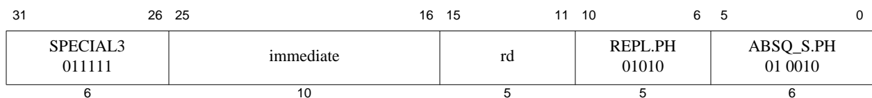
Figure 5-4 SPECIAL3 Encoding for the ABSQ_S.PH instruction sub-class with the immediate field
