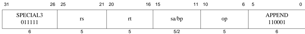
Figure 5.12 SPECIAL3 Encoding for the APPEND instruction sub-class
