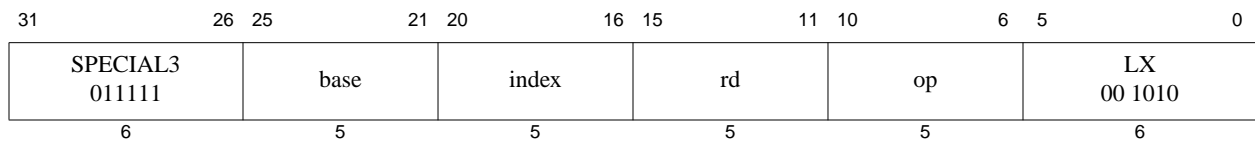
Figure 5-6 SPECIAL3 Encoding for the LX instruction sub-class
