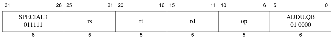
Figure 5-2 SPECIAL3 Encoding for the ADDU.QB/CMPU.EQ.QB instruction sub-classes
