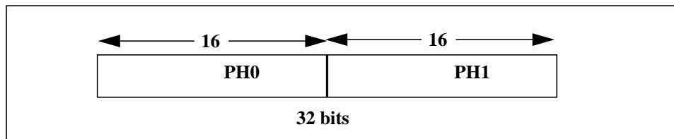
Figure A-2 The Big-Endian PH0 and PH1 Elements in a GPR for the MIPS32® Architecture
