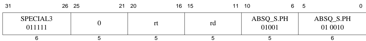
Figure 5-3 SPECIAL3 Encoding for the ABSQ_S.PH instruction sub-class without immediate field
