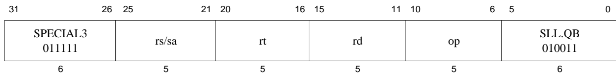
Figure 5-5 SPECIAL3 Encoding for the SHLL.QB instruction sub-class
