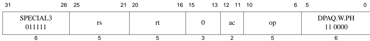
Figure 5-7 SPECIAL3 Encoding for the DPAQ.W.PH instruction sub-class
